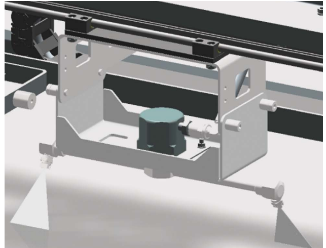
High-pressure cleaning system of the HUBER Drum Screen LIQUID.
