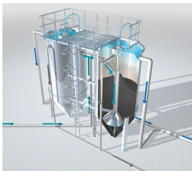
HUBER Active Carbon Filter CONTIFLOW® GAK (tank design).
