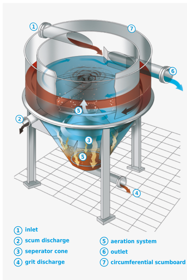
Flow diagram of a HUBER Circular Grit Trap HRSF.
