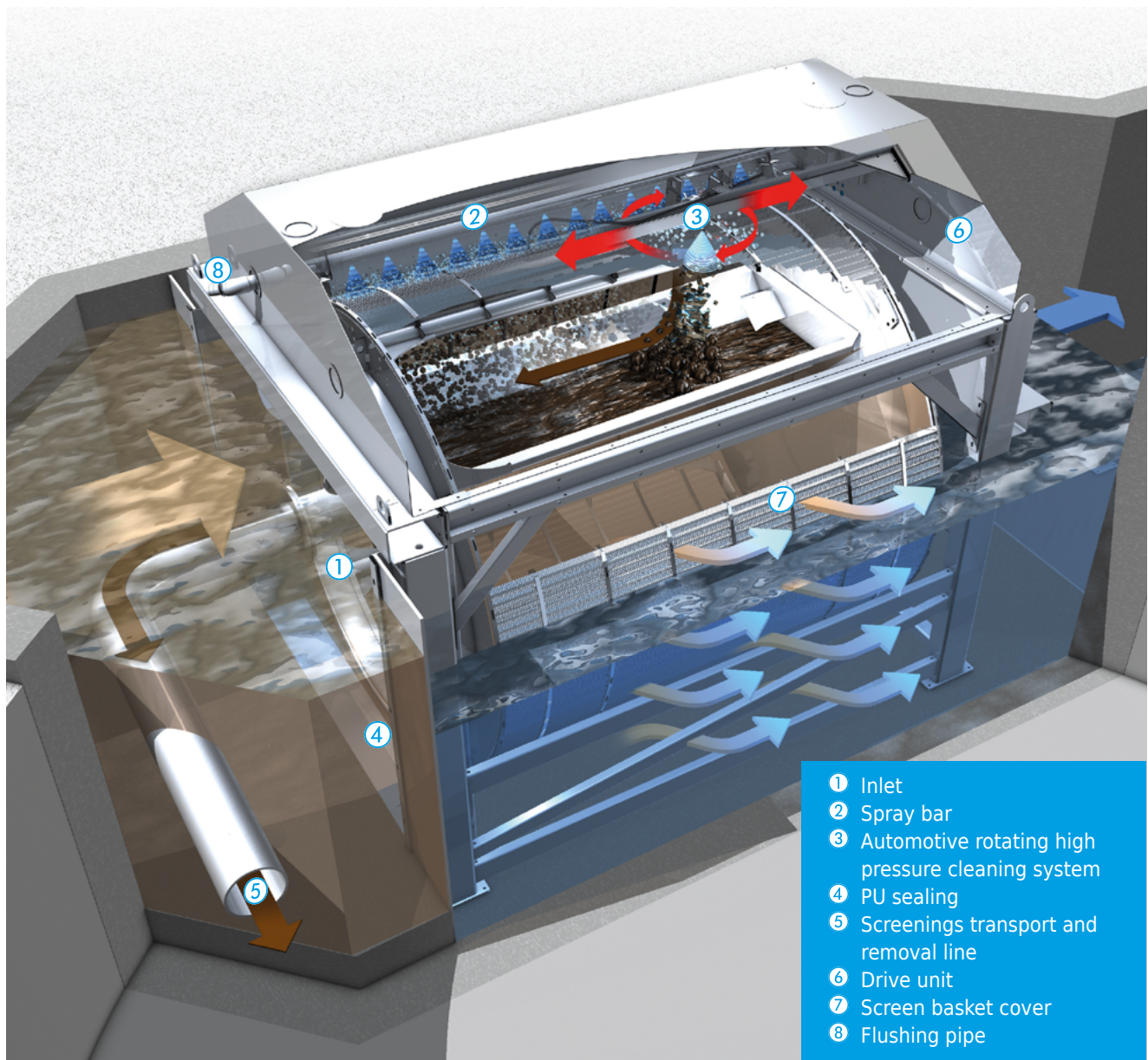
HUBER Drum Screen LIQUID for channel installation.
