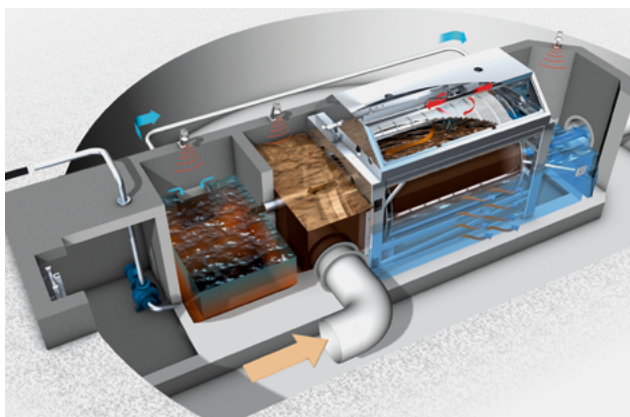
CarbonWin® process illustration: The better preliminary clarifier tank for optimum reduction rates (see individual brochure).
