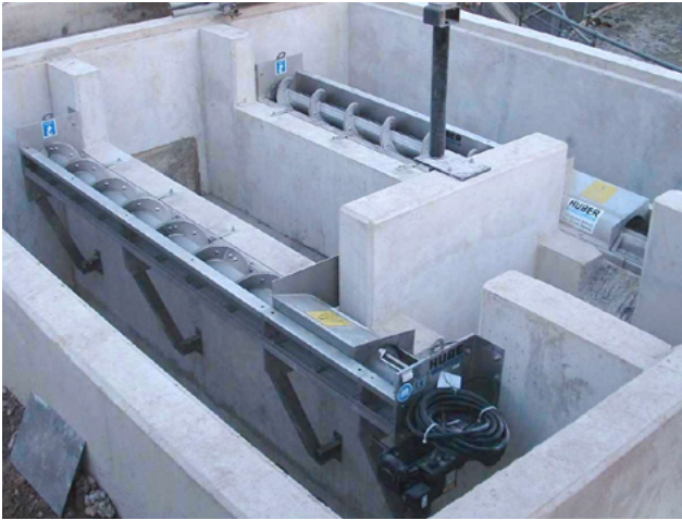
ROTAMAT® RoK1 Storm Screens on both sides of an overflow, combined with dissipation and flow control.
