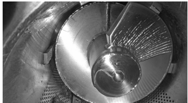
A screw shaft beginning to wear.
